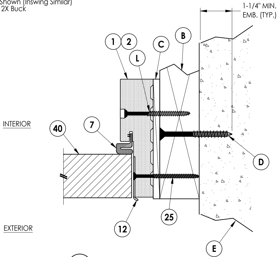
2 HORIZONTAL CROSS SECTION 3 Outswing Shown (Inswing Similar) Shown w/ 2X Buck
